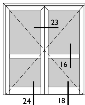
ΔΙΦΥΛΛΗ ΑΝΟΙΓΟΜΕΝΗ ΕΞΩ DOUBLE LEAF DOOR OPENING OUTSIDE
